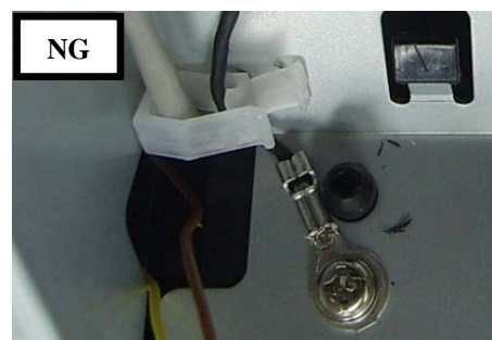
FG cable and shield wire are not close enough.
