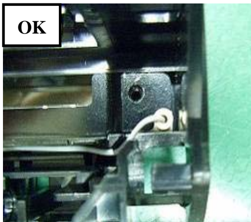
The reflector steps on the rubber on the lamp socket.
