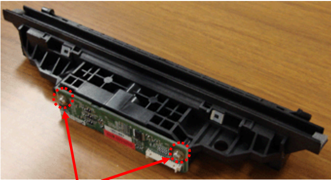
CCD board fixing screw (x2)
