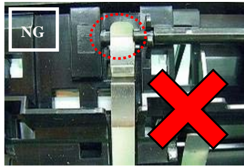
Not thread the plate through the Revolve frame hole. When installing the Feed FG Plate, do not insert the plate into a wrong hole.
